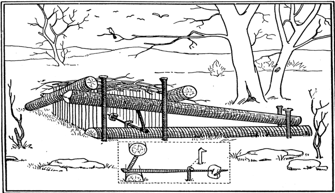
TWO PIECE' TRIGGER TRAP.
