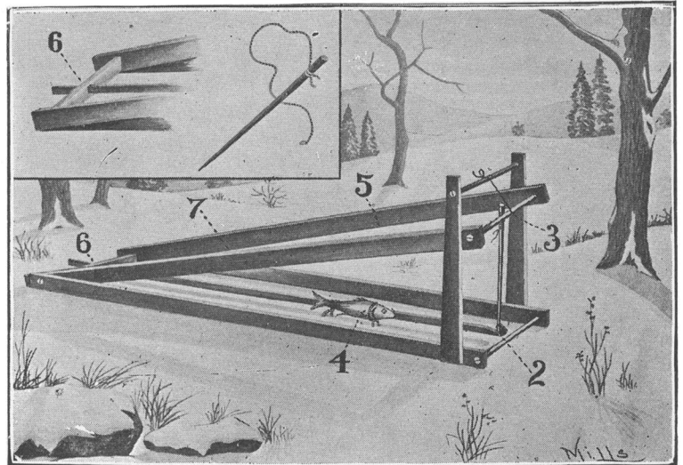
PORTABLE WOODEN TRAP.
