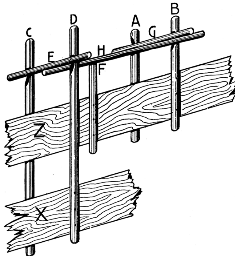
MARTEN DEADFALL.
