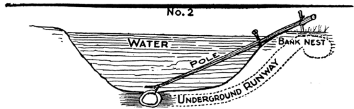
UNDERGROUND RAT RUNWAY.
