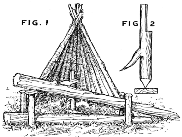
THE TURN TRIGGER.
