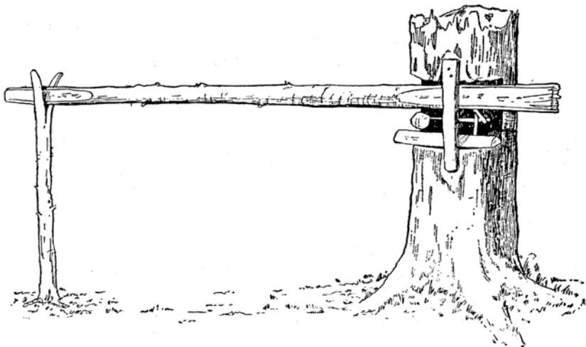
TREE DEADFALL.
