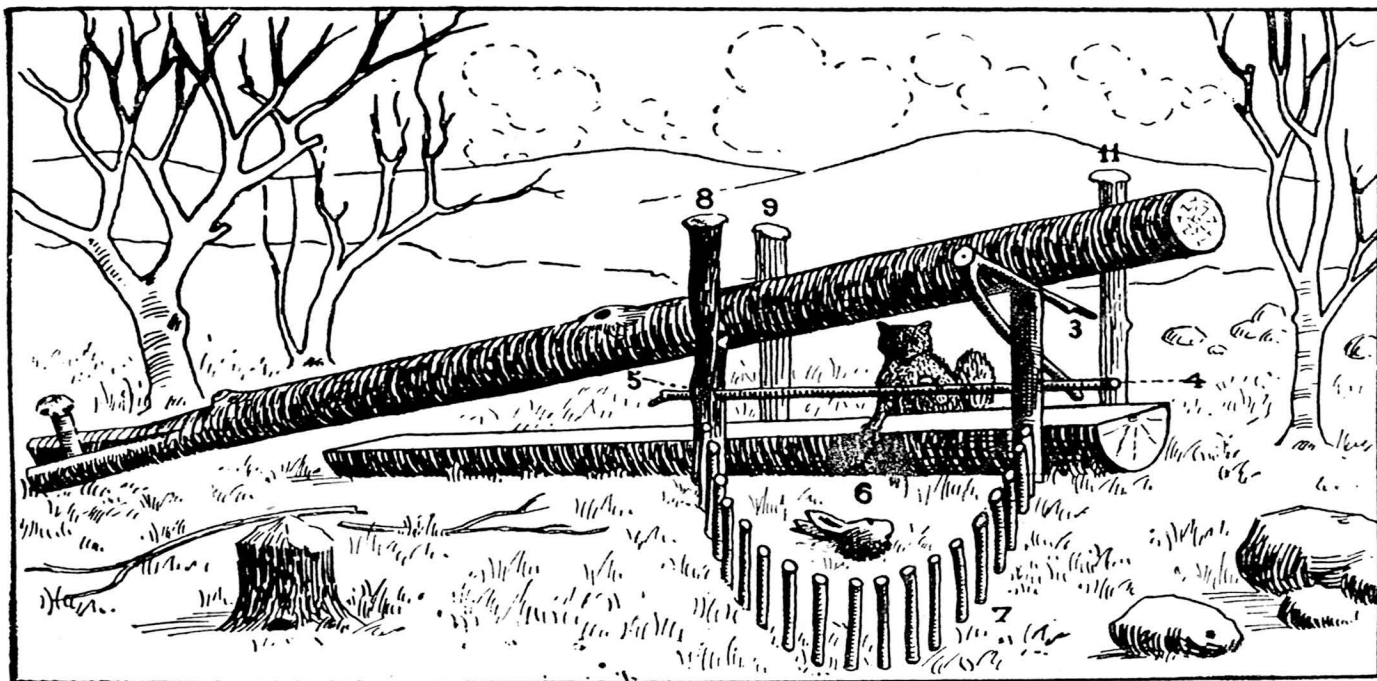
ANIMAL ENTERING TRIP DEADFALL.
