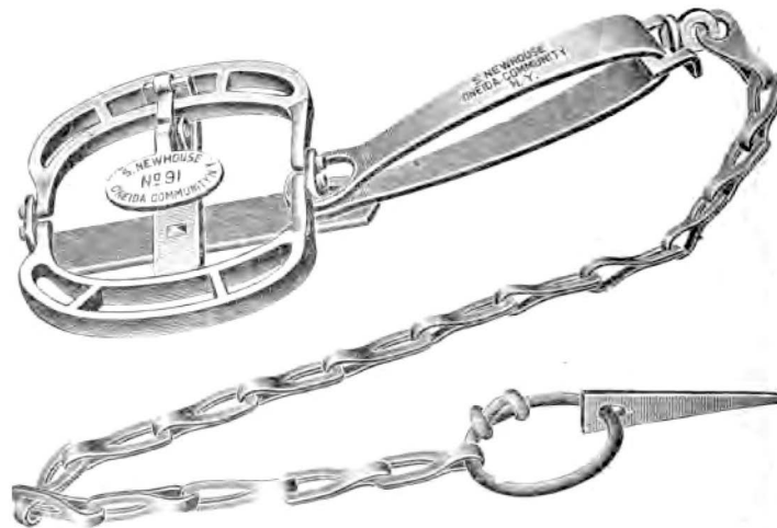
Spread of Jaws--91, 5¼ inches : 91½, 6¼ inches
