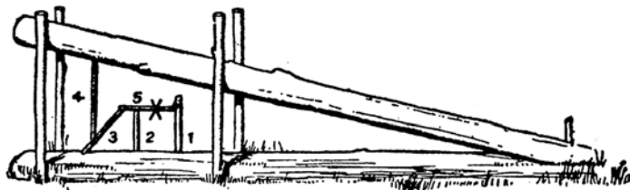
ILLINOIS TRAPPER'S TRIGGERS.
