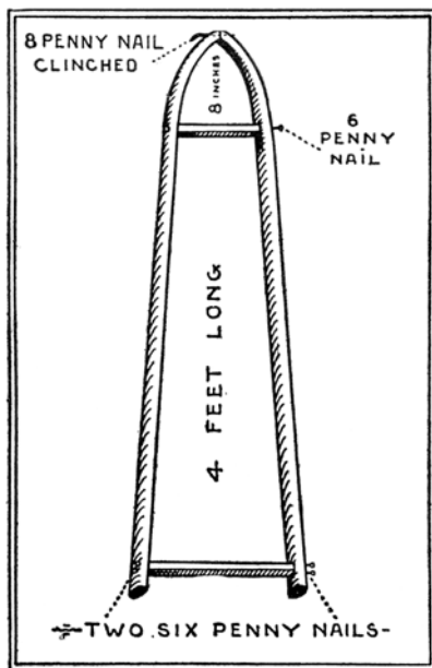
STRETCHING FRAME.
