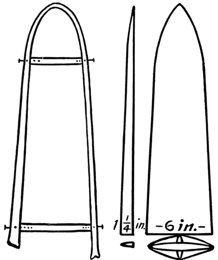
POLE STRETCHERS.
