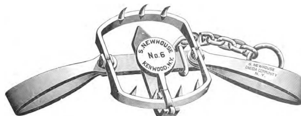
Spread of Jaws, 16 inches. Weight, complete, 42 pounds
