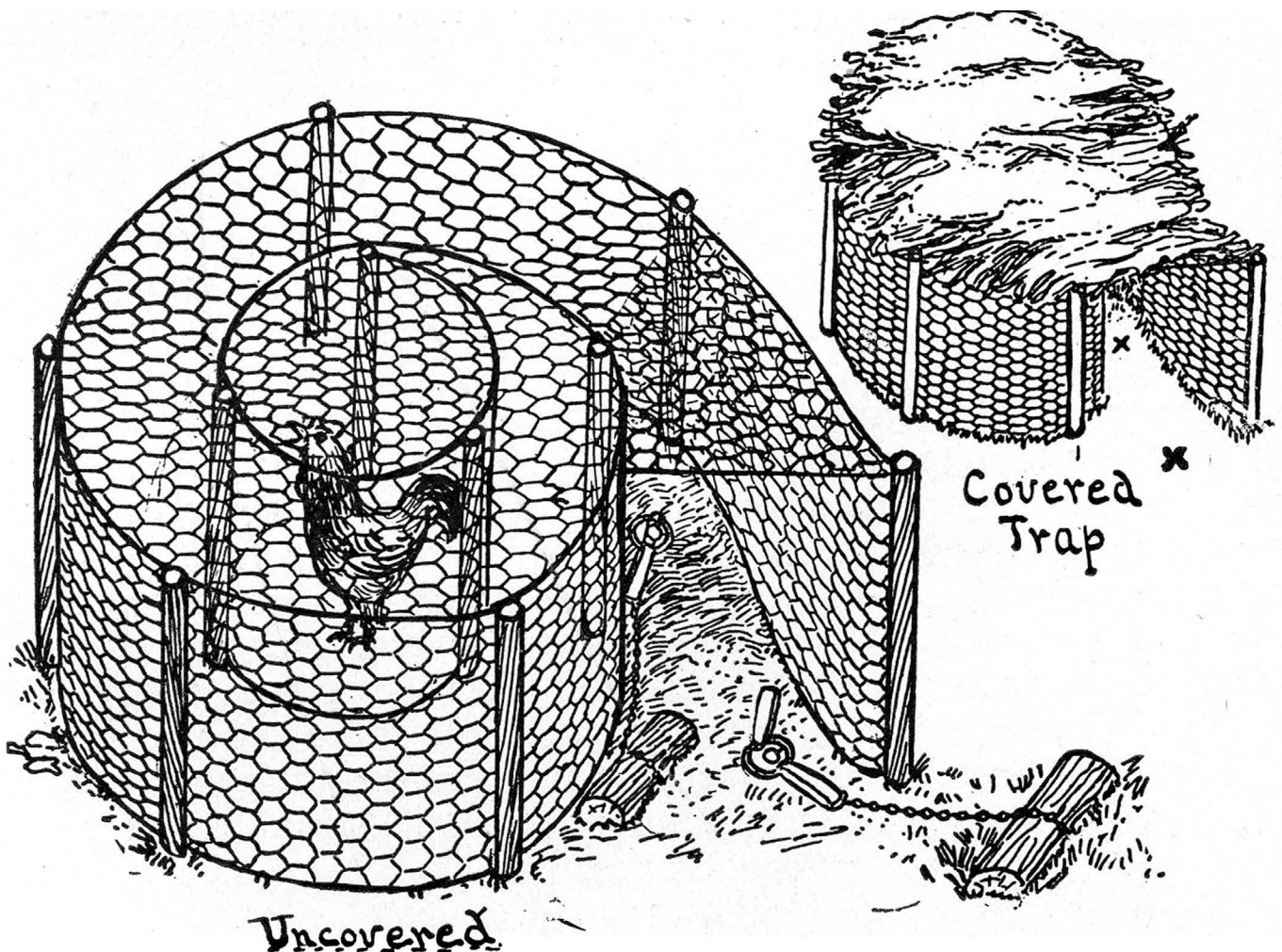
SCREENED ROOSTER TRAP.
