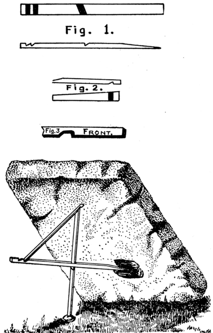
STONE DEADFALL TRIGGERS.
