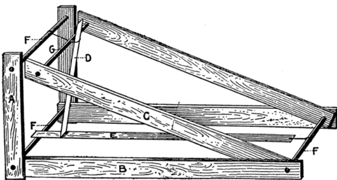
THE NOX-EM-ALL DEADFALL.
